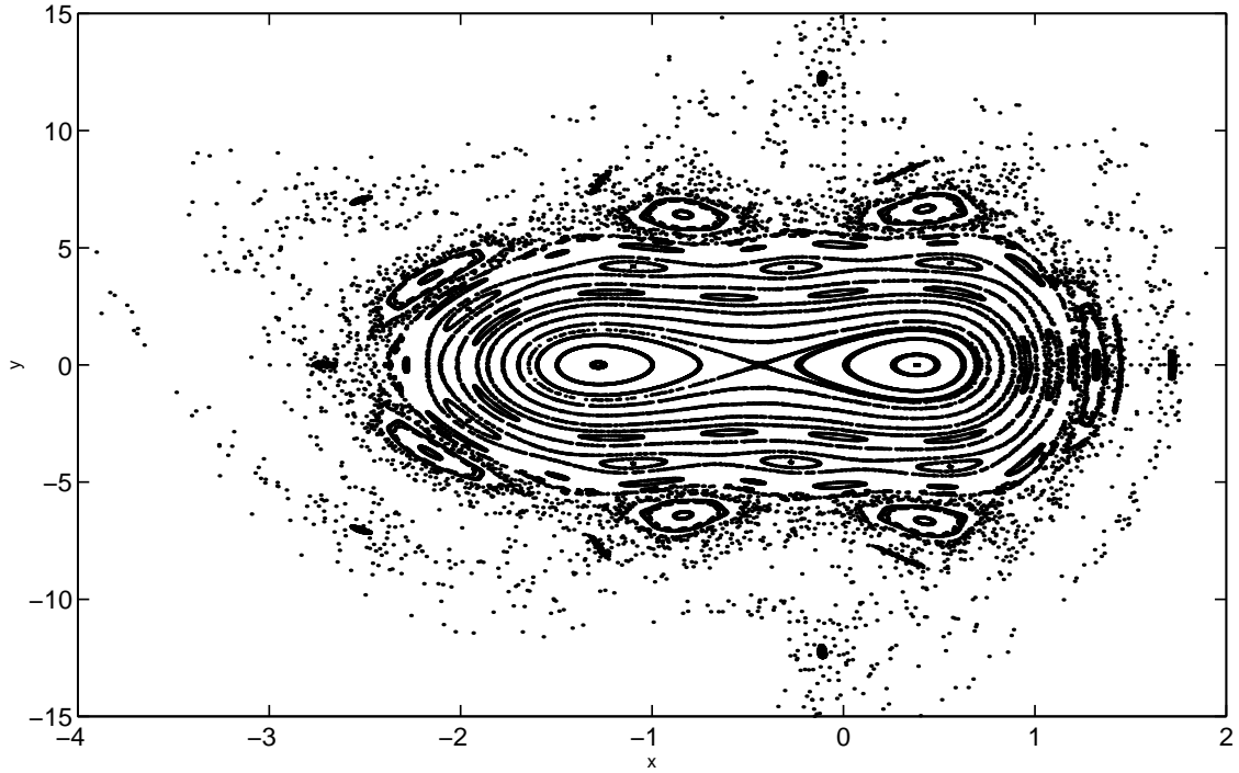
FIGURE 1. A Poincaré plot for parameter values \alpha = -10 and E = 10 . Reproduced from [4]
