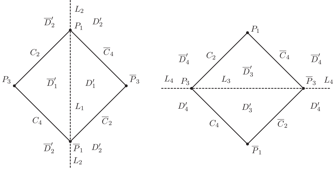
FIGURE 1. The 8 cones meeting at singularities of \tilde{Z} . The broken lines are the images of the four G -invariant twistor lines, which separate D_j and \bar{D}_j for 1 \leq j \leq 4 . The rational curves C_j, \bar{C}_j, j = 2, 4 and L_j, 1 \leq j \leq 4 , are the intersection of the corresponding divisors.
