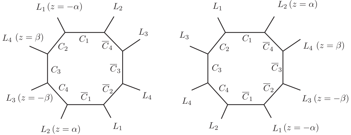
FIGURE 2. Octagons formed by the 8 torus-invariant rational curves and the configuration of torus-invariant twistor lines. The left figure is for one of the two incorrect small resolutions, and the right figure is for one of the two correct small resolutions.
