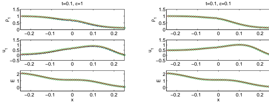
Figure 5: Example 5.2, at t=0.1 , we compare the results give by the Exp-RK method (the dotted line), the BGK penalization method (the circled line) and the reference solution (the solid line). The left figures are for \varepsilon=1 , and the right ones are for \varepsilon=0.1 .
