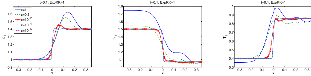
Figure 2: Example 5.1, as \varepsilon goes to zero, the results get to the Euler limit, i.e. a stationary shock.
