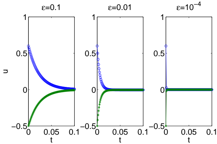
Figure 7: Example 5.2, the velocities converge to the mean velocity at different rates for different \varepsilon 's. The circled line stands for species one, and the dotted line stands for species two. The smaller \varepsilon gives the faster convergence rate.
