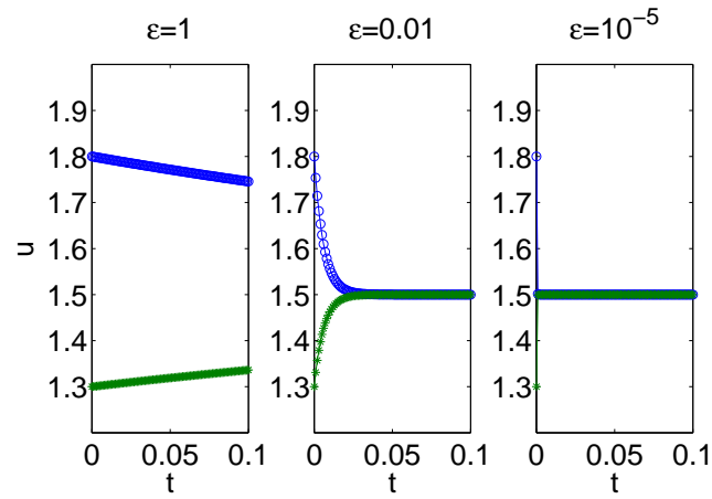
Figure 3: Example 5.1, the velocities converge to the mean velocity at different rates for different \varepsilon 's. The circles and dots stand for the velocities of the first and second species respectively. The smaller \varepsilon gives the faster convergence rate.
