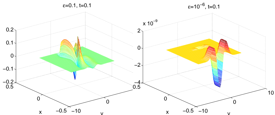
Figure 8: Example 5.2, f - M for \varepsilon = 1 and \varepsilon = 10^{-6} at t = 0.1 .
